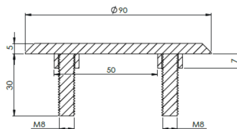
SECTION A-A SCALE 1.2:1
